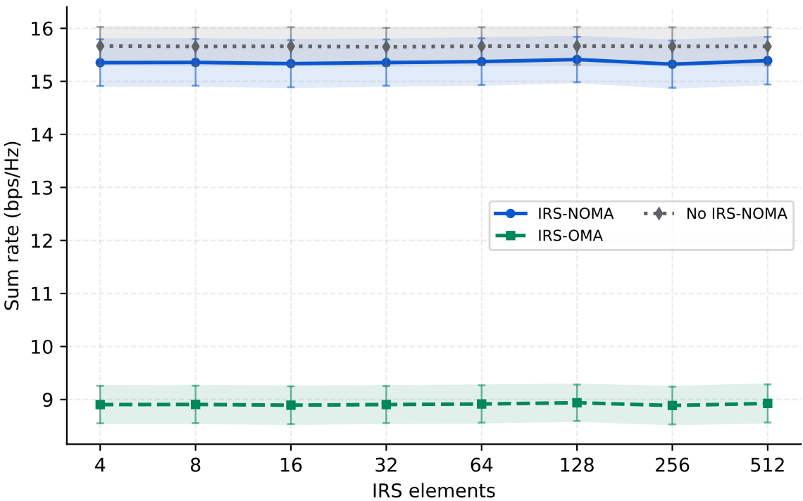
NOMA Sum Rate versus IRS Elements
