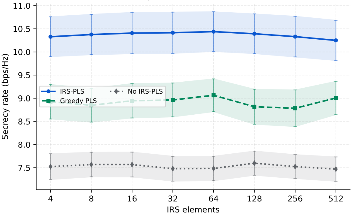
Secrecy Rate versus IRS Elements
