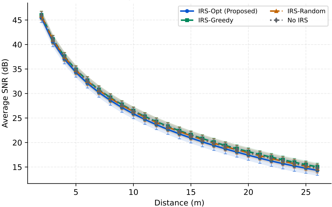
Average SNR versus Tx-Rx Distance
