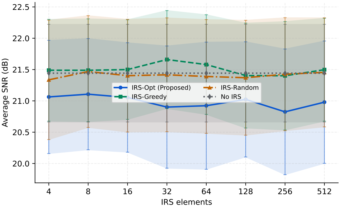
Average SNR versus IRS Elements
