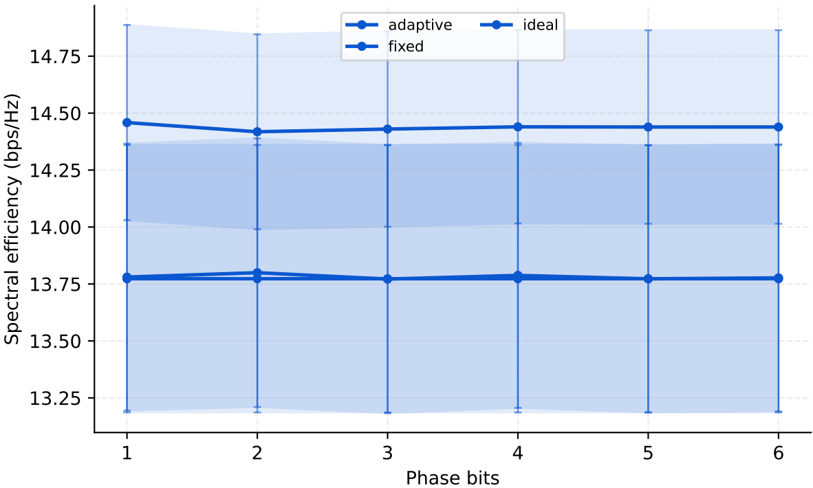
Spectral Efficiency versus Phase Resolution
