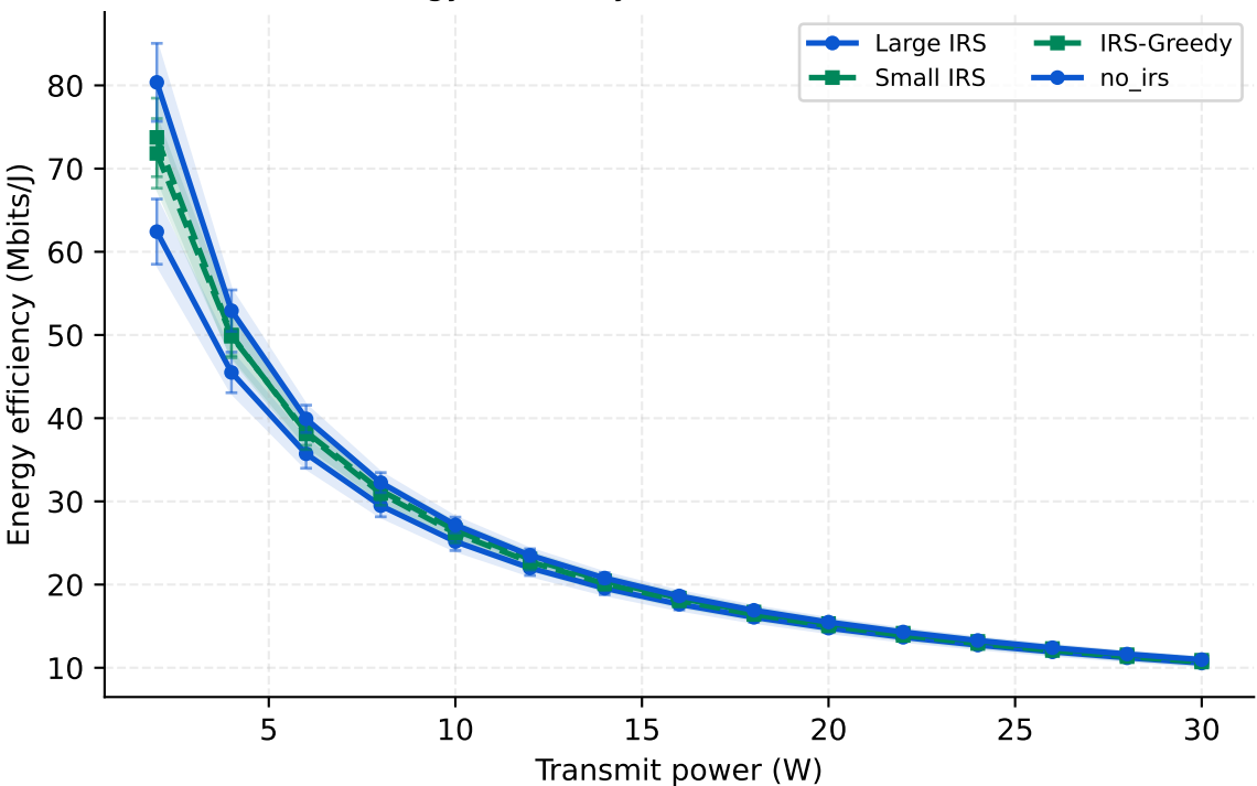
Energy Efficiency versus Transmit Power
