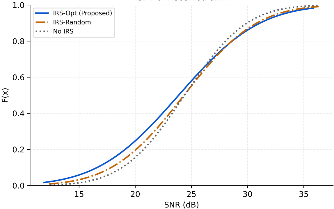
CDF of Received SNR
