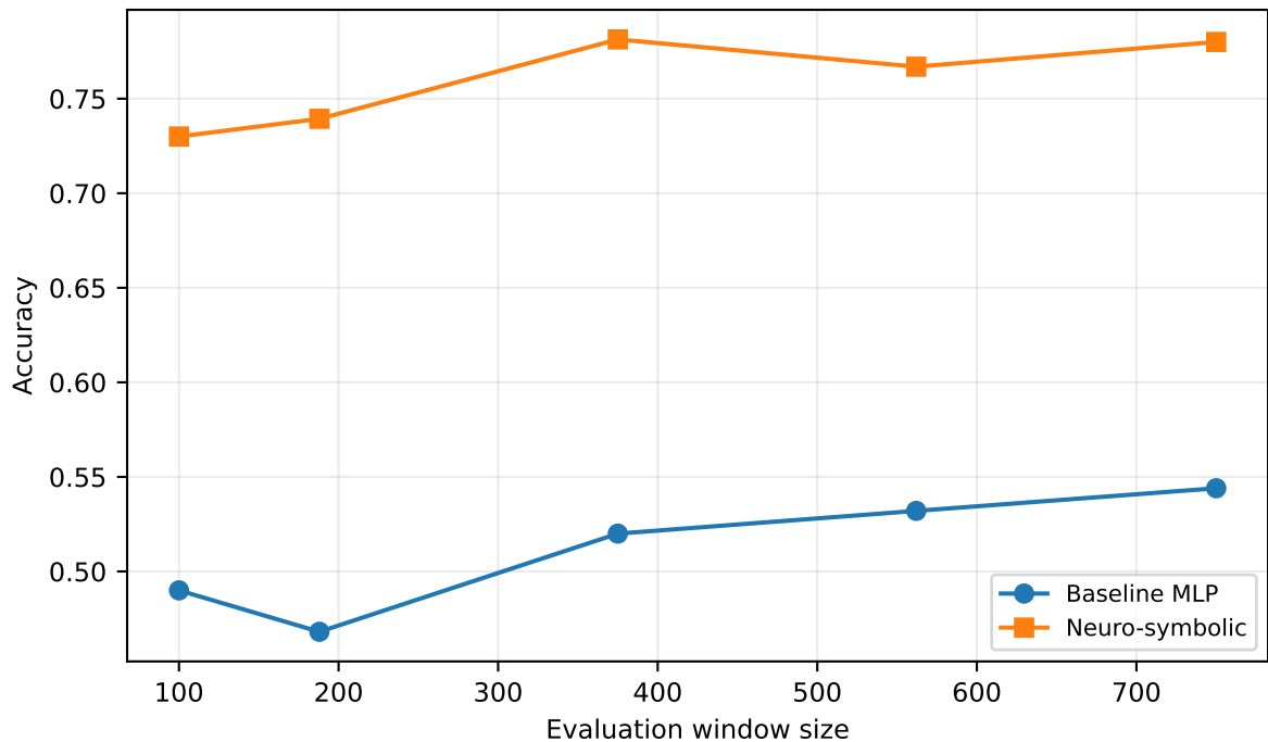
Accuracy Improvement Curve
