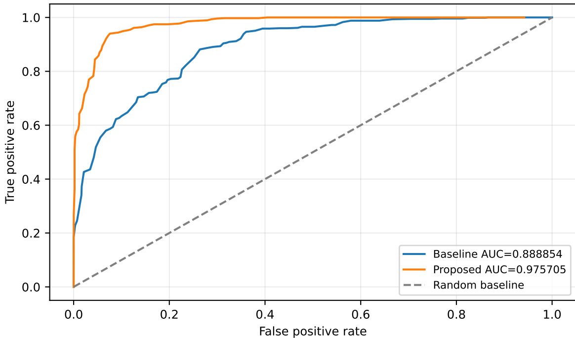
Micro-Average ROC Curve
