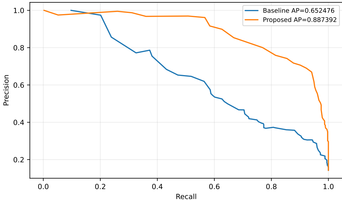
Micro-Average Precision-Recall Curve
