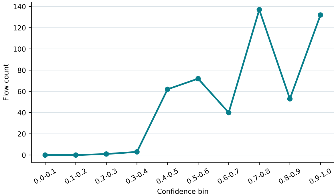
Prediction Confidence Distribution
