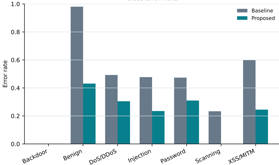
Class Error Rate
