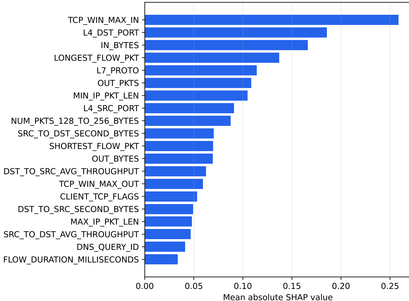
Global Feature Importance
