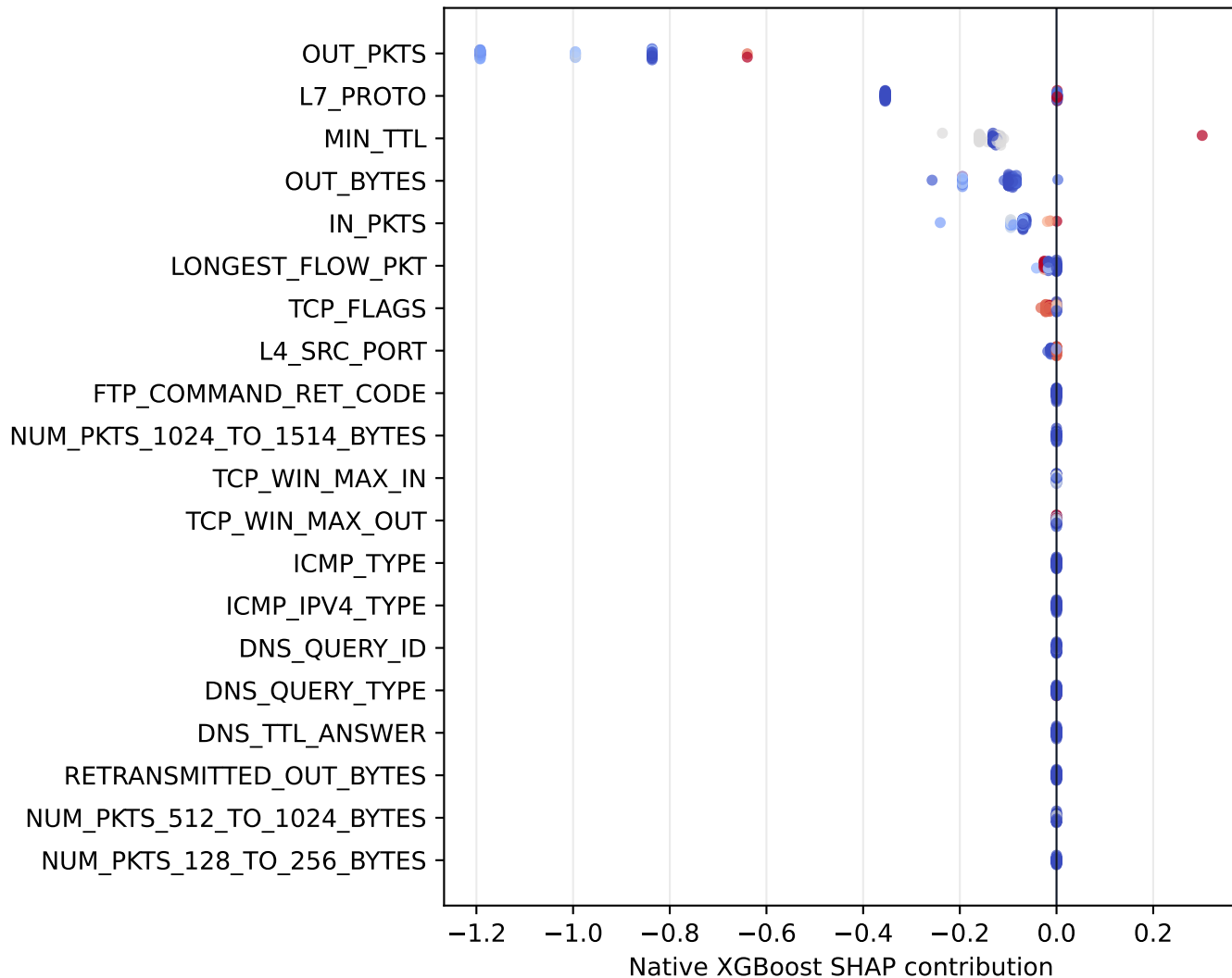
SHAP Beeswarm
