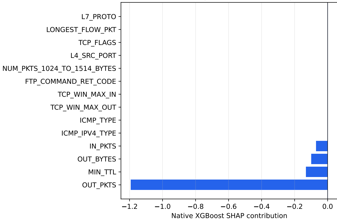
SHAP Waterfall Sample: base=0.422, output=-1.069
