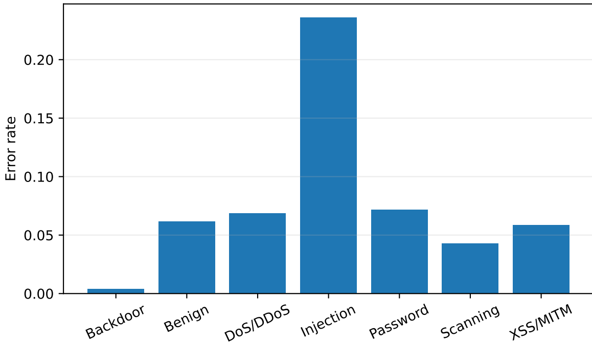
Class Error Rate
