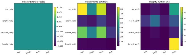
Fig. 4. Integrity suite summary. All targets returned exit code 0 (zero errors) across sequential, random 4 KB, and random 64 KB verification profiles. ArcFS shows higher wall-clock runtime on fsync4k_verify due to user-space flush cost per sync point, a structural property of the FUSE architecture.
