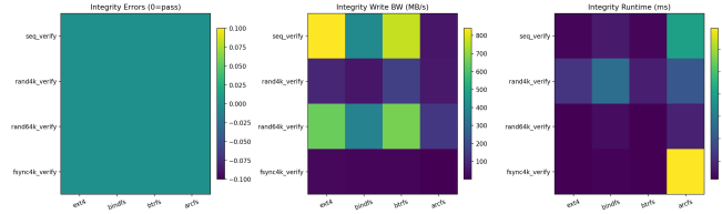
Figure 4: Integrity suite summary. All targets returned exit code 0 (zero errors) across sequential, random 4 KB, and random 64 KB verification profiles. ArcFS shows higher wall-clock runtime on fsync4k_verify due to user-space flush cost per sync point, a structural property of the FUSE architecture.
