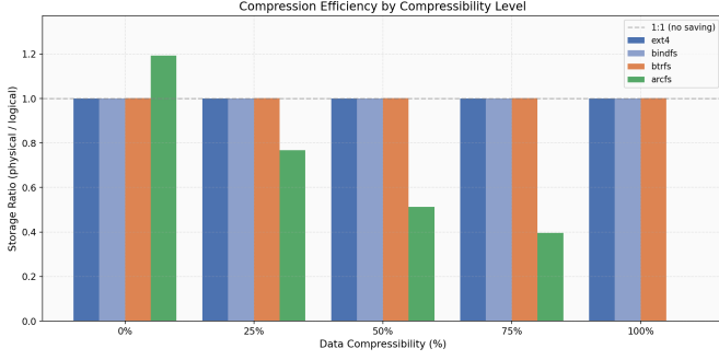
Figure 6: Physical-to-logical storage ratio versus data compressibility (0% = pure random bytes; 100% = uniform zeros). Ext4, bindfs, and uncompressed Btrfs hold a 1.0 ratio at all levels. ArcFS achieves 0.77 at 25%, 0.51 at 50%, and 0.396 at 75% compressibility. Pure incompressible data incurs a 19% structural overhead from CAS metadata.
