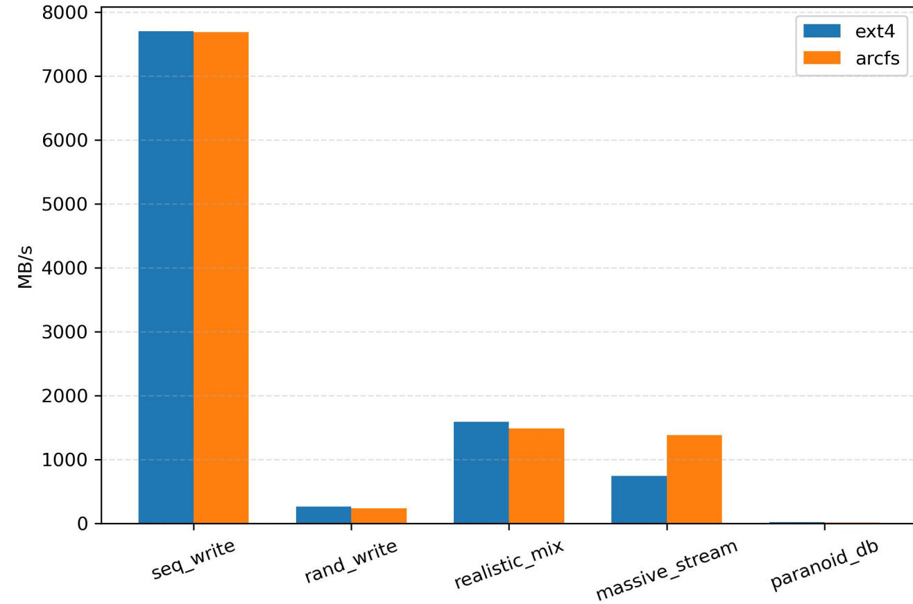
Durable: ArcFS vs ext4 Write BW
