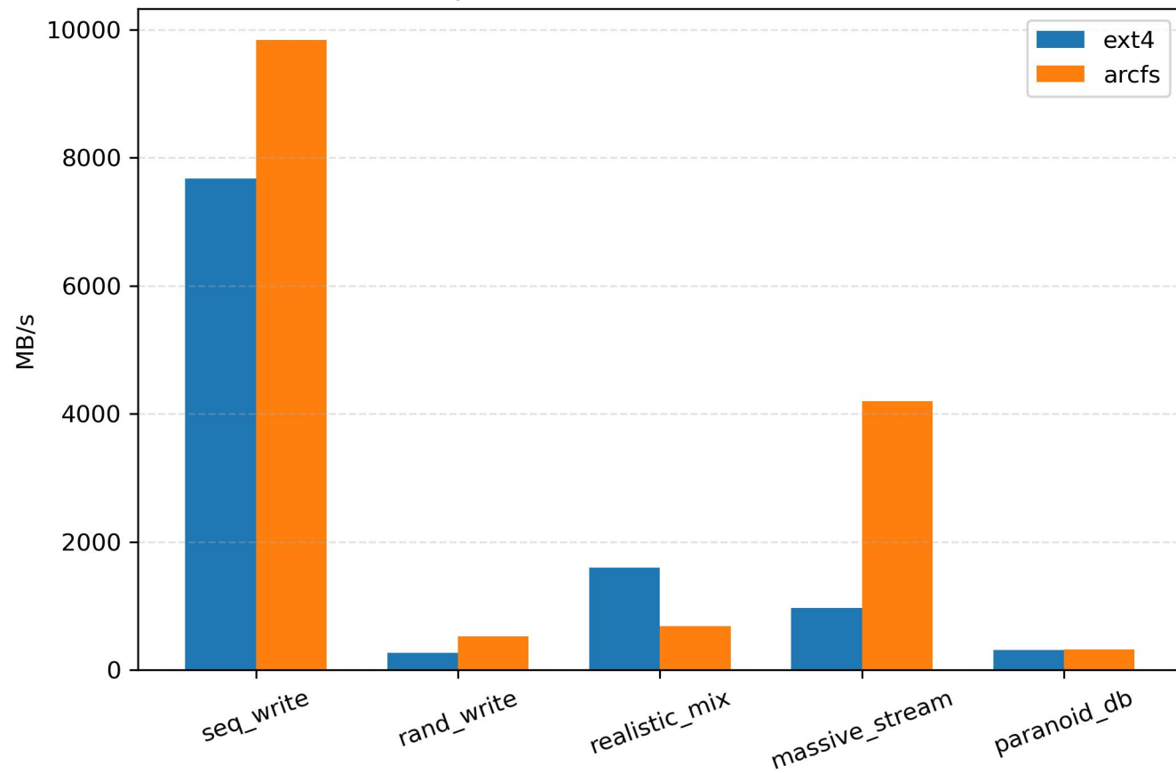
Responsive: ArcFS vs ext4 Write BW
