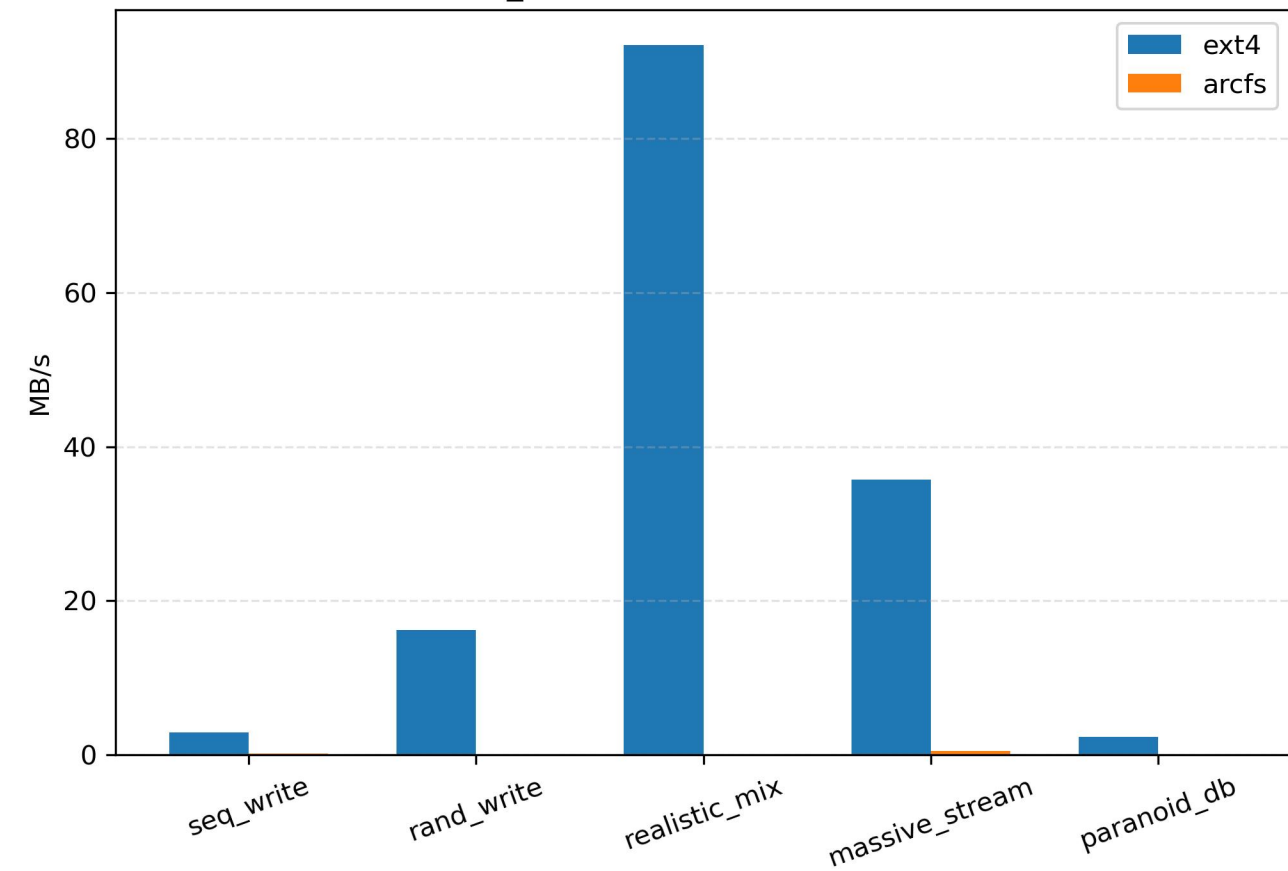
Worst_case: ArcFS vs ext4 Write BW
