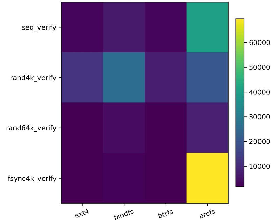
Integrity Runtime (ms)
