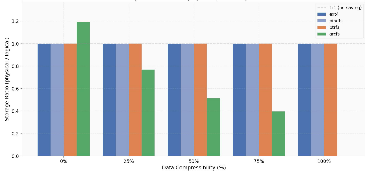
Compression Efficiency by Compressibility Level
