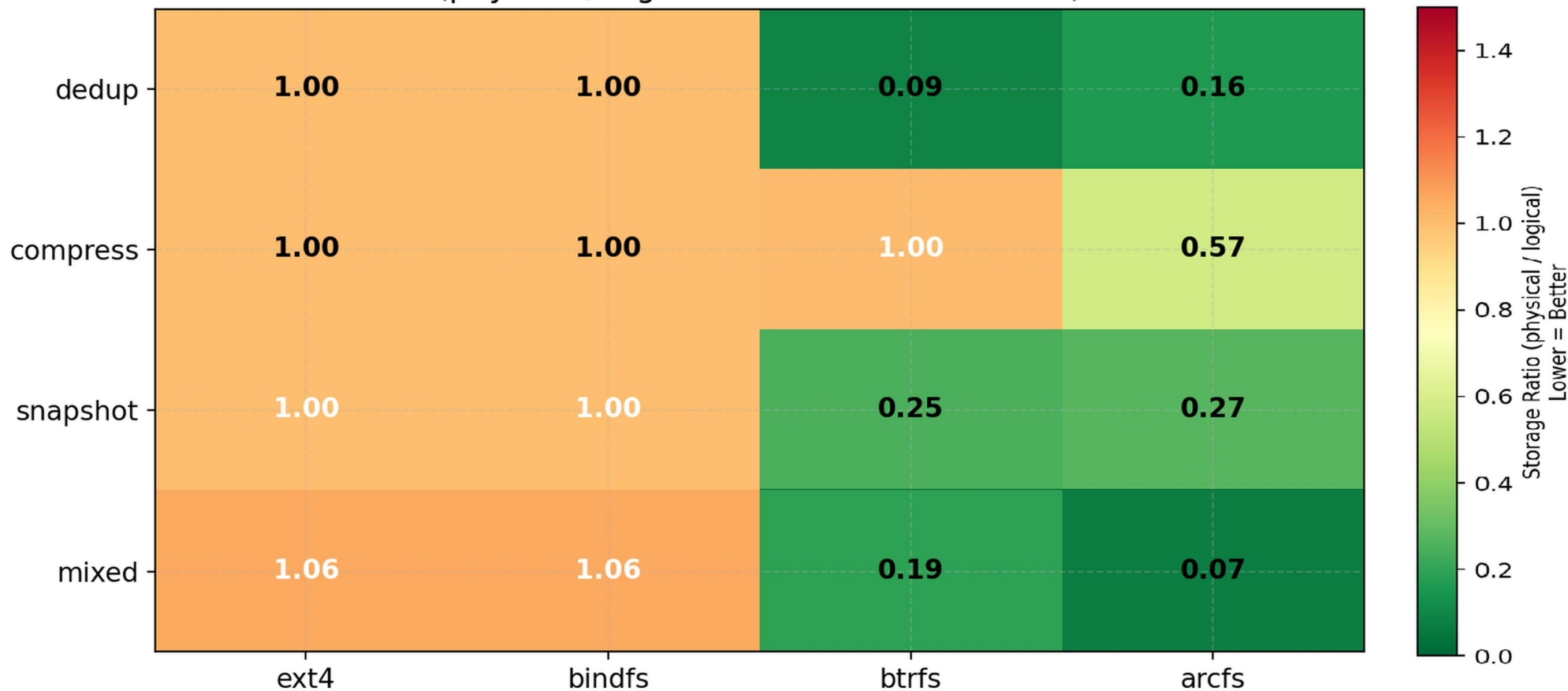
Disk Usage Efficiency Summary (physical / logical ratio — lower is better)
