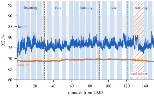
Fig. 3. Evening session on the dry enclosure, lid 4 cm (blue shading: mist reaching the enclosure). Both controllers mist most of the time; the hatched window is the injected dead mister.
