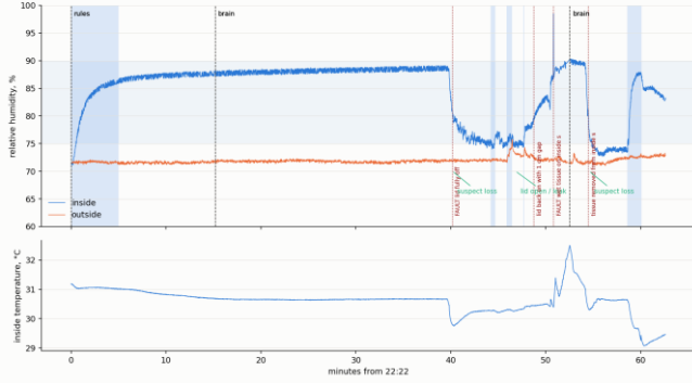
Fig. 3. Fault session: humidity (top) and inside temperature (bottom); dotted red lines mark injected events, green labels the controller's verdicts.
