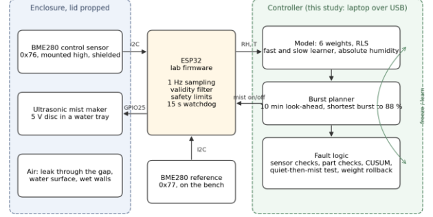
Fig. 1. System: enclosure, ESP32 laboratory firmware and the controller with its three functions; in this study the controller ran on a laptop over USB.
