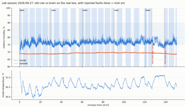
Fig. 5. Alternating session, evening, dry enclosure: both controllers mist most of the time; the dotted lines mark the software dead-mister window in the last block.
