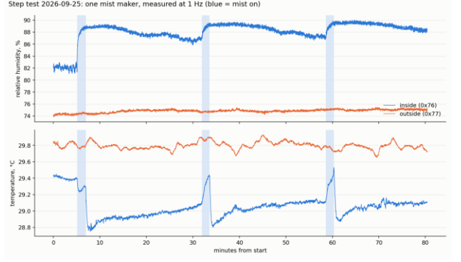
Fig. 2. Step test: inside and outside humidity (top) and temperature (bottom) over three mist rounds; shaded bands mark mist on.
