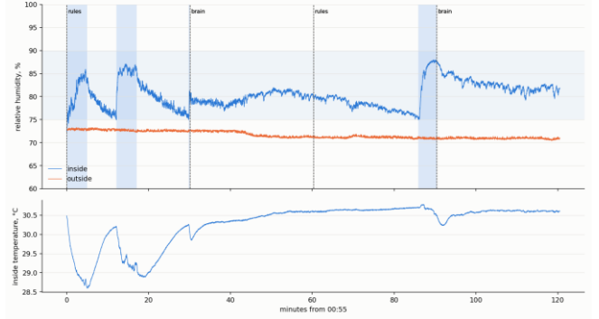
Fig. 4. Alternating session, night: the rule mists to its 300 s cap whenever the enclosure reaches 75 %; the learning controller, judging the enclosure's own equilibrium sufficient, never mists.
