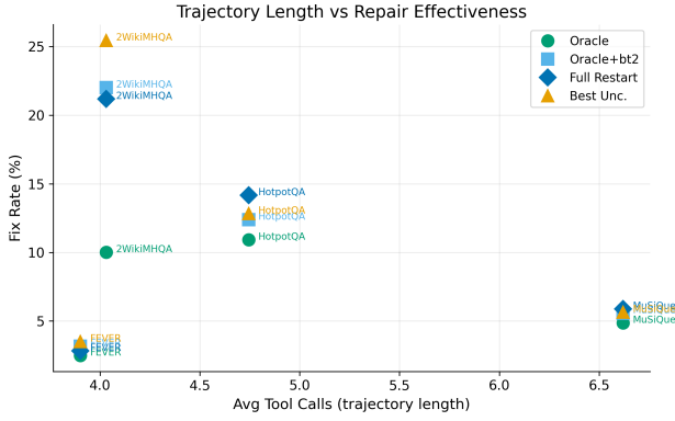
Figure 4: Trajectory length vs. repair effectiveness. Shorter trajectories (FEVER, 2WikiMHQA) favor targeted repair; longer trajectories (HotpotQA, MuSiQue) favor full restart, consistent with the context contamination hypothesis.
