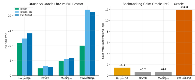
Figure 2: Left: Oracle, Oracle+bt2, and Full Restart fix rates. Right: Backtracking gain (Oracle+bt2 – Oracle). The +12.0 pp gain on 2WikiMultiHopQA confirms strong error cascade effects.
