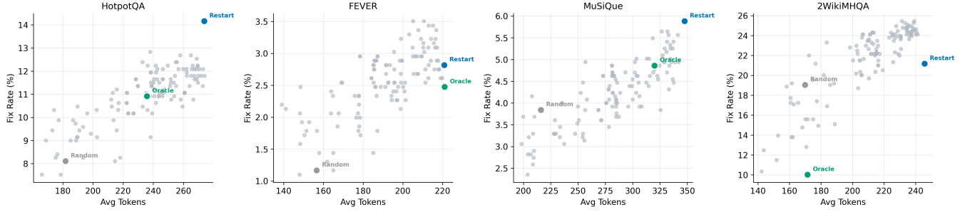
Figure 5: Cost-accuracy Pareto fronts for all four datasets. Each grey dot is an individual repair strategy; labeled points show baselines. On 2WikiMultiHopQA, many uncertainty strategies dominate the Pareto front above Full Restart.
