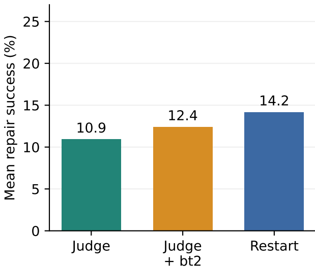
HotpotQA
