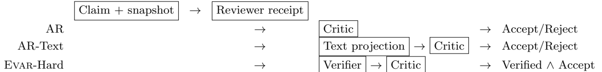
Figure 1: Matched protocol flow. All variants use the same reviewer and critic call count; only EVAR-Hard makes deterministic verification a necessary gate.
