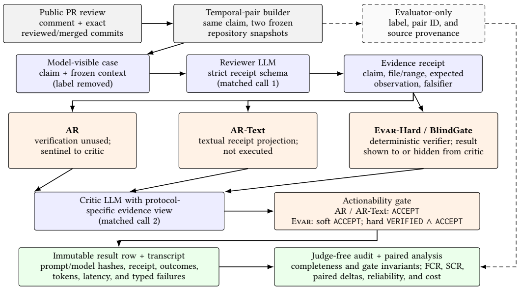
Fig. 1. Whole EVAR architecture. Public review history becomes a temporally paired benchmark case while labels remain evaluator-only. The reported design shows verification to the EVAR-Hard critic; the powered BlindGate control withholds it and derives paired soft/hard decisions from the same row. Every attempt produces an immutable record for judge-free audit, decision metrics, reliability, and cost accounting.
