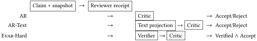
Fig. 1. Matched protocol flow. All variants use the same reviewer and critic call count; only EVAR-Hard makes deterministic verification a necessary gate.
