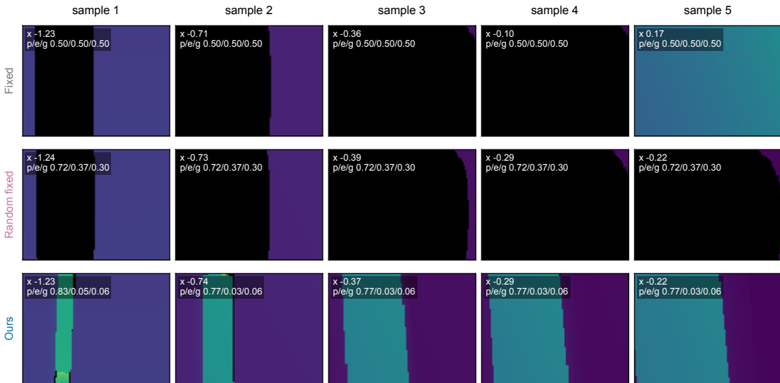
Observed depth along each method's own closed-loop trajectory: glare, slot=far_right
