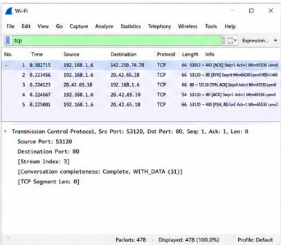
3. TCP Filter Applied (tcp)
