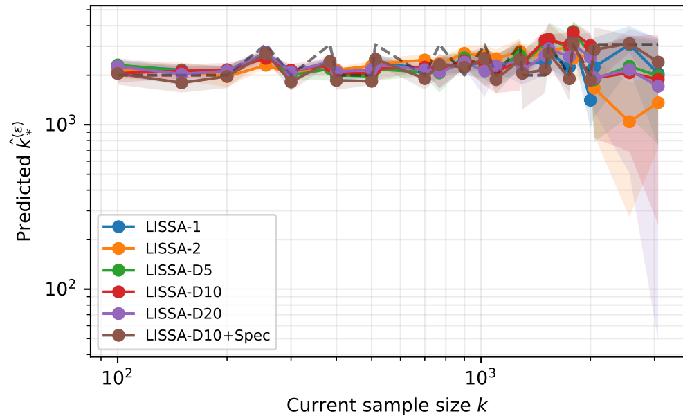
Aggregated sufficiency predictions over repeated splits ( \varepsilon = 0.02 )
