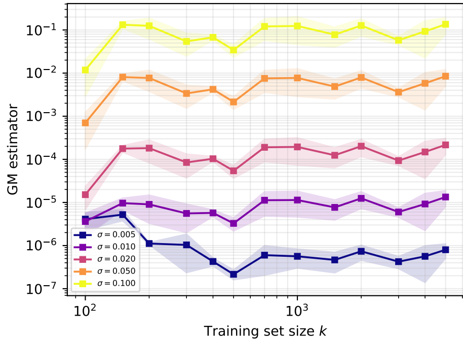
Gaussian-moment proxy
