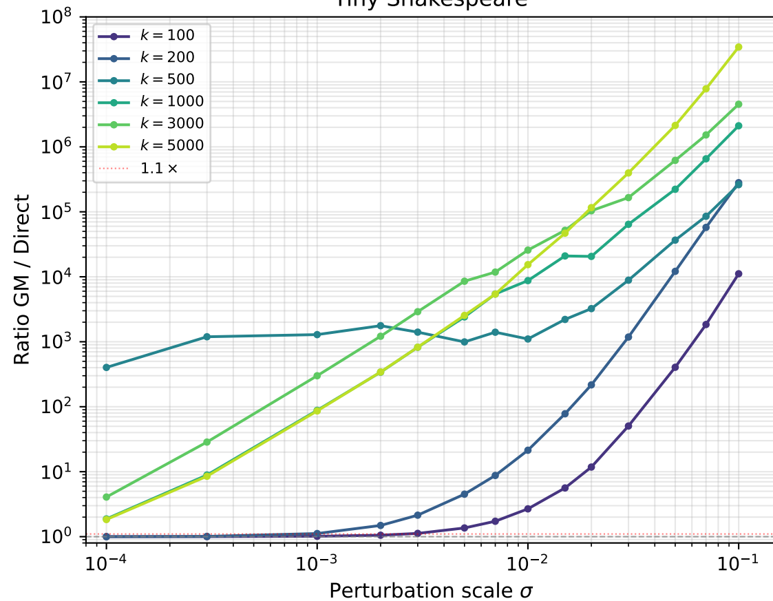
Tiny Shakespeare
