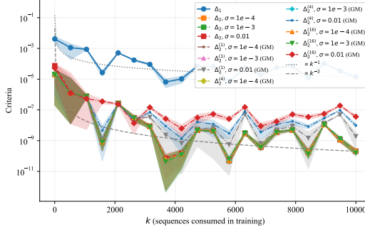
Figure 2: Decay of stabilization criteria with sample size. Comparison of \Delta_1 , \Delta_2 , and \Delta_2^{(D)} as functions of k .
