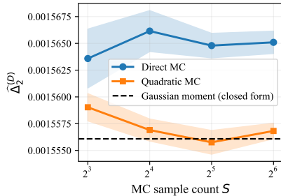
Figure 5: Convergence of Direct MC and Quadratic MC estimates of \hat{\Delta}_2^{(D)} to the Gaussian-moment closed form as the sample count S increases, at D = 10 and \sigma = 10^{-3} .
