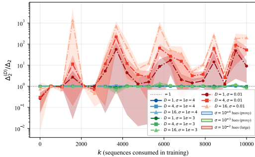
Figure 3: Subspace criterion relative to the full-space criterion. Ratio \Delta_2^{(D)}/\Delta_2 across sample size k , for several dimensions D and scales \sigma .
