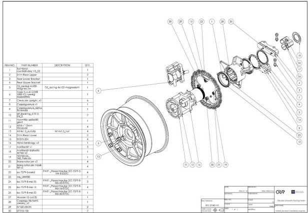
Assembly drawing, 30 item BOM
