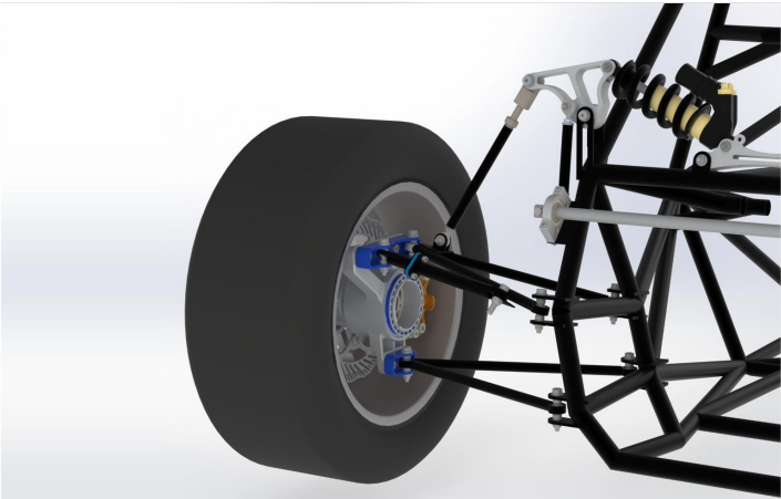
01 Suspension
