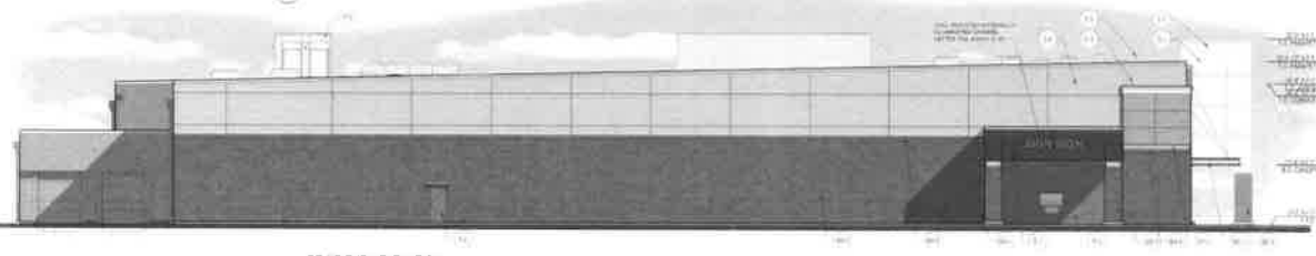
DRIVE-THRU ELEVATION 44% MASONRY / 56% NON-MASONRY
