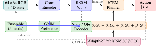
Figure 1. System overview. The agent observes, encodes, updates the RSSM posterior, and plans via iCEM with multi-component EFE scoring. Adaptive precision dynamics modulate \beta weights based on state prediction errors and obstacle proximity.
