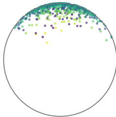
Concentrated vMF
