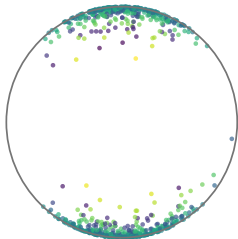
Opposed modes
