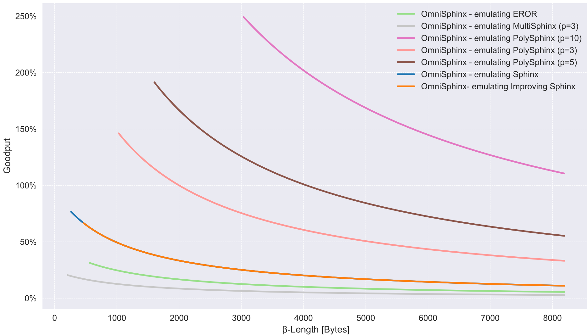
Goodput as a Function of \beta
