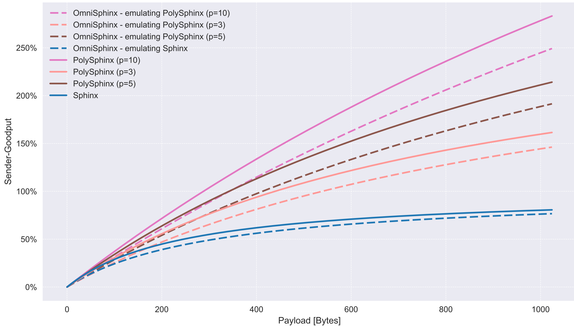
Sender-Goodput for PolySphinx variants
