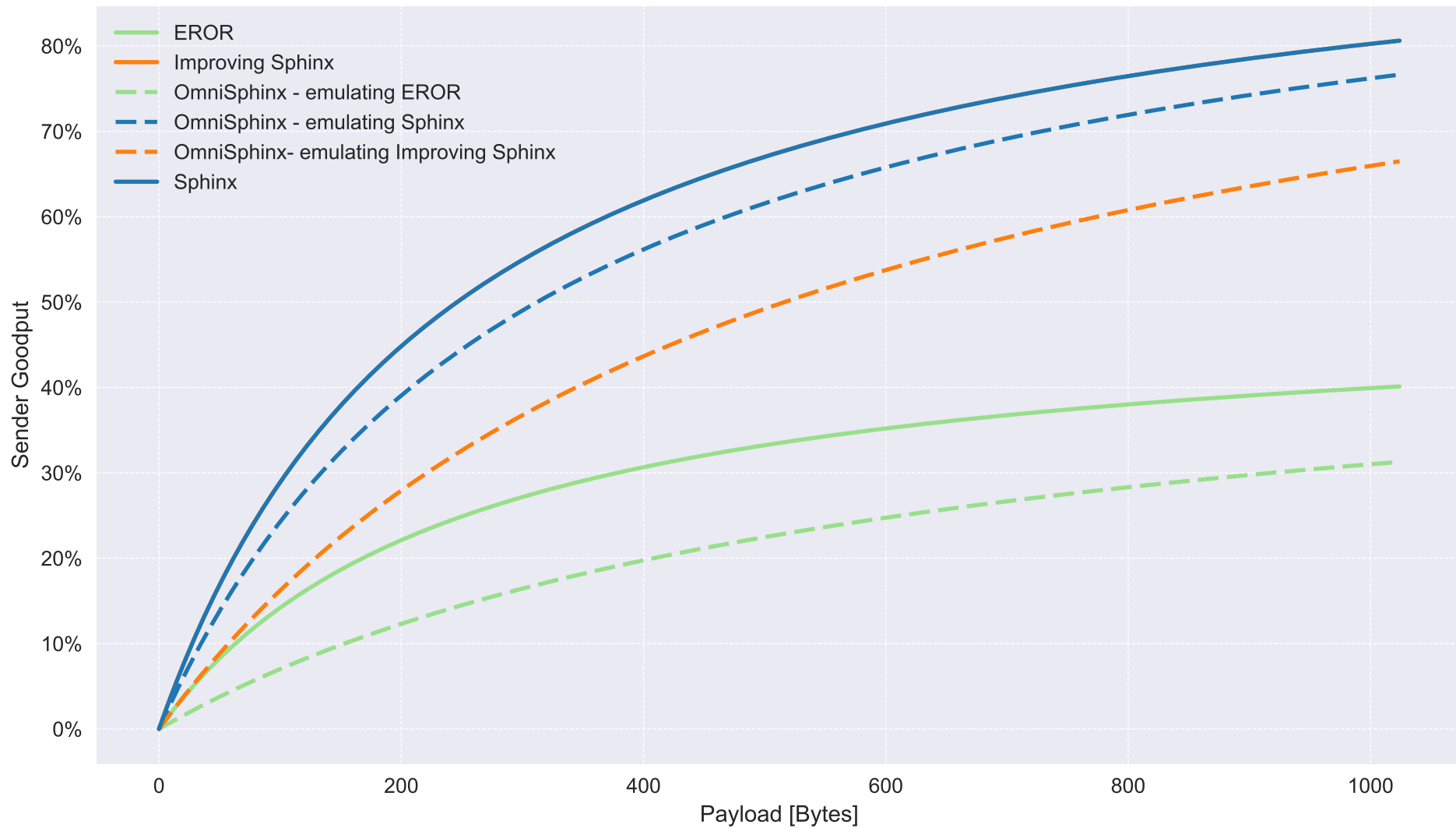
Sender Goodput for OmniSphinx variants with minimal \beta
