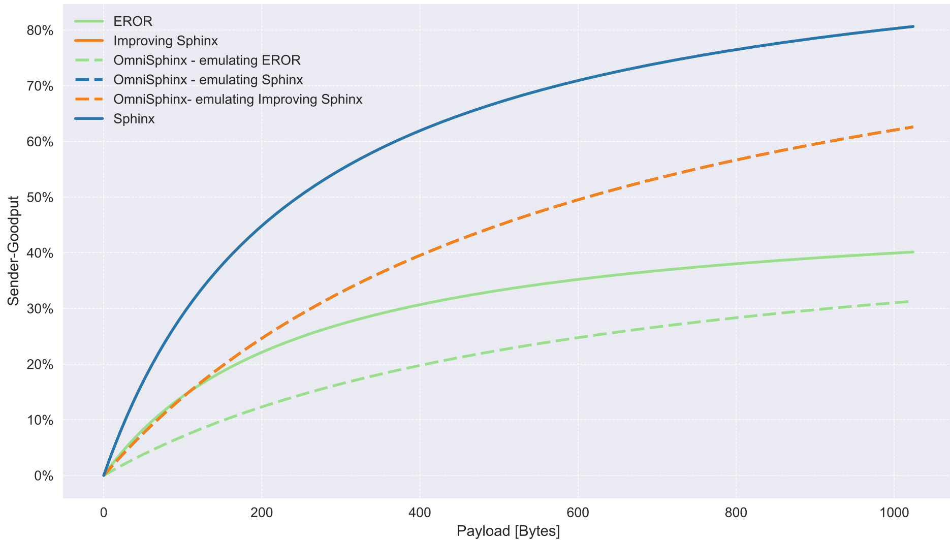
Sender Goodput for OmniSphinx variants with EROR \beta
