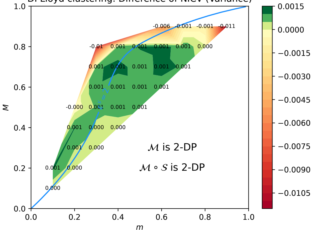
DPLloyd clustering: Difference of NICV (Variance)
