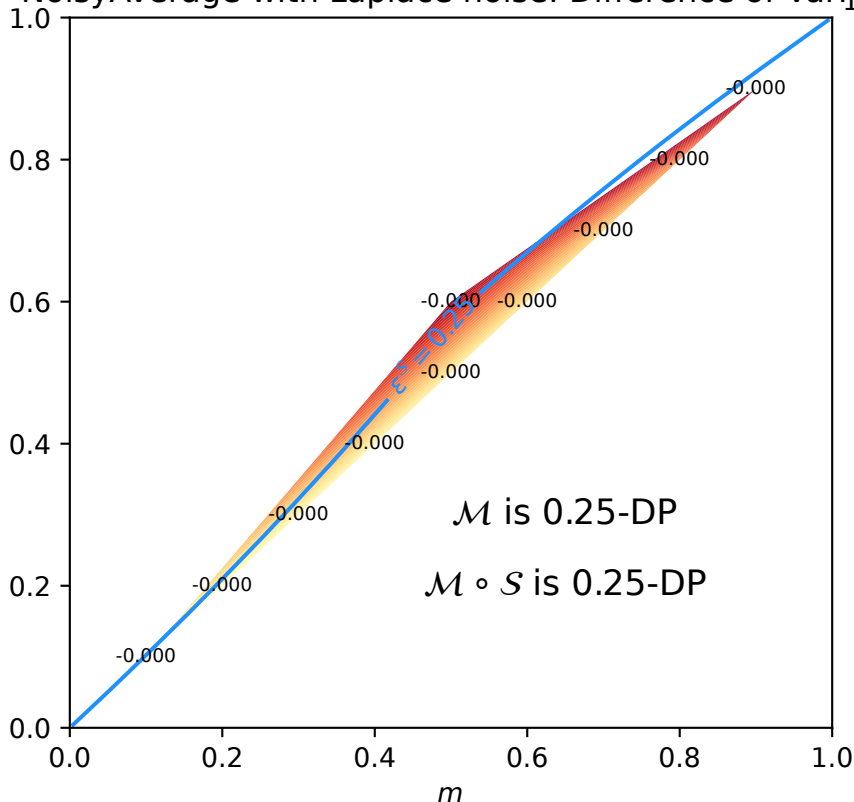
NoisyAverage with Laplace noise: Difference of VarRE
