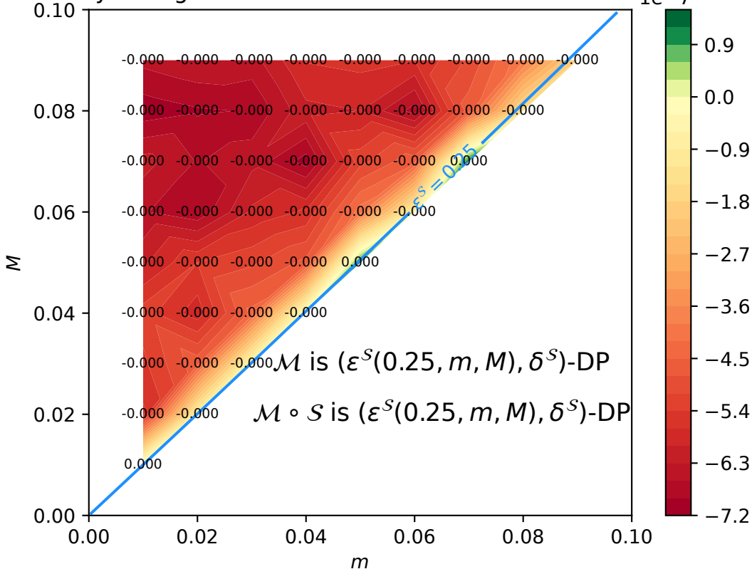
NoisyAverage with Gaussian noise: Difference of \text{Var}(\text{RE}_7)
