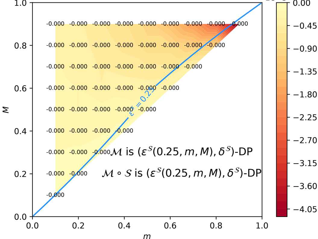
NoisyAverage with Gaussian noise: Difference of VarPE 5
