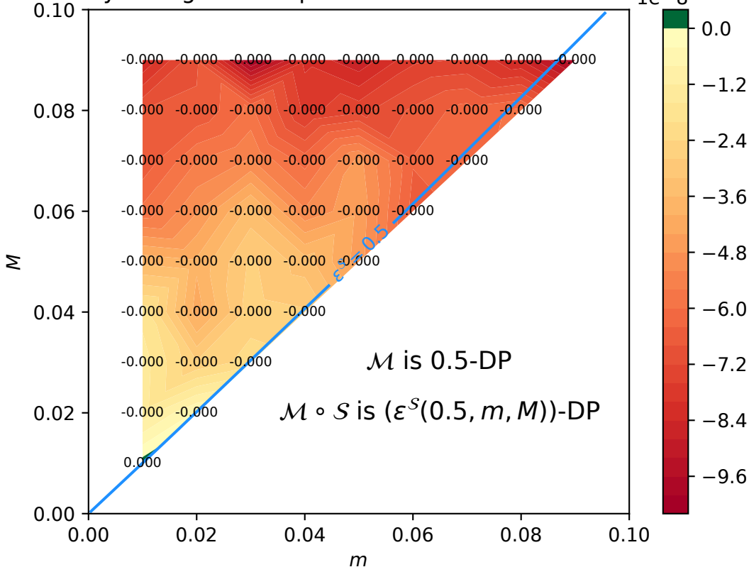
NoisyAverage with Laplace noise: Difference of VarRE 1e-8
