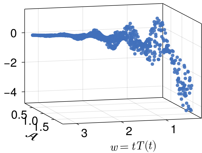
\tau = 1.0 \text{ fm}/c
