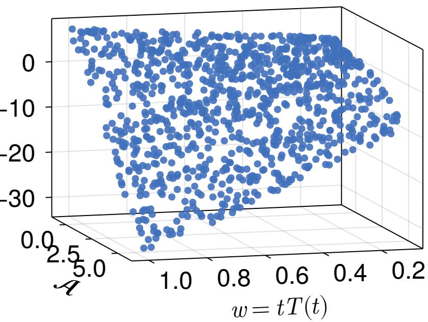
\tau = 0.45 \text{ fm}/c
