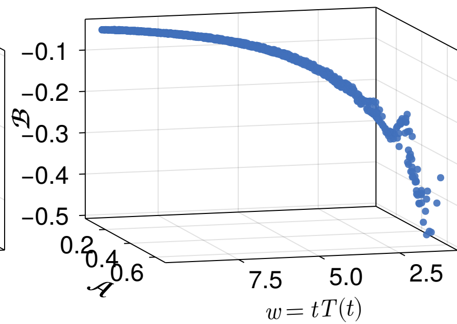
\tau = 5.0 \text{ fm}/c
