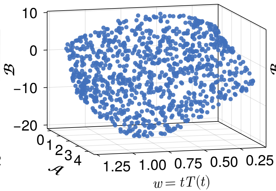
\tau = 0.55 \text{ fm}/c
