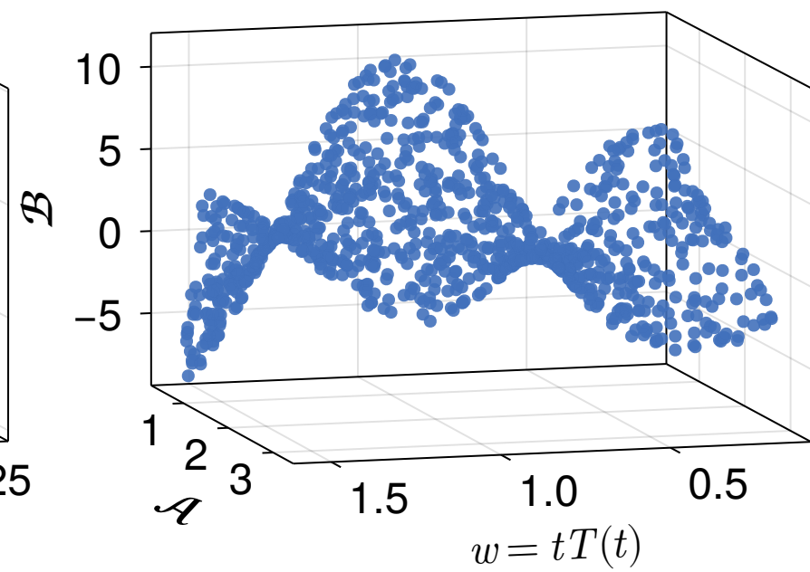
\tau = 0.65 \text{ fm}/c
