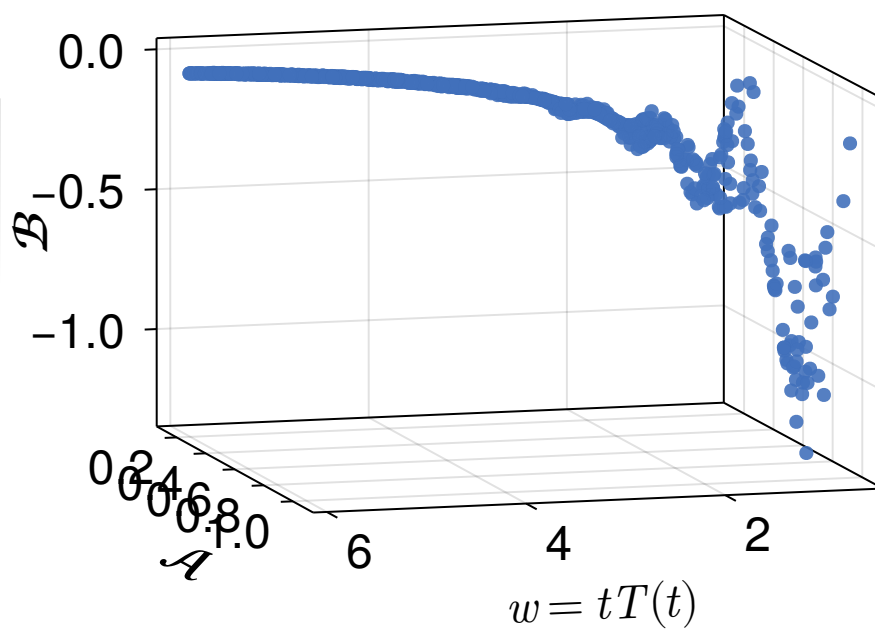
\tau = 2.5 \text{ fm}/c
